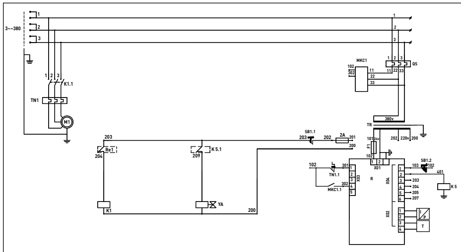
Fig. 2.4 Electrical diagram A07., AR07., ARD07..*
