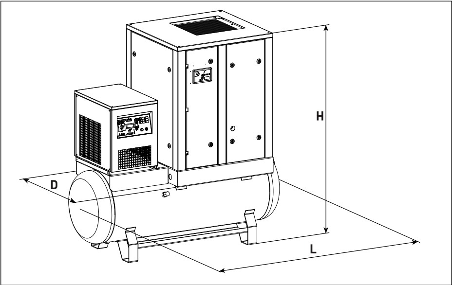
Fig. 3.4 Dimension drawing AR07..-AR22, ARD07..-ARD22
