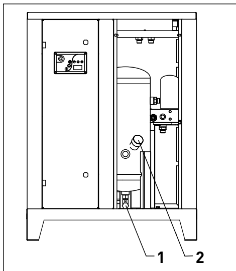
Fig. 5.3 Oil replacing
