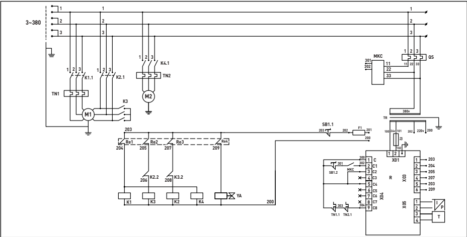
Fig. 2.6 Electrical diagram A30-55
